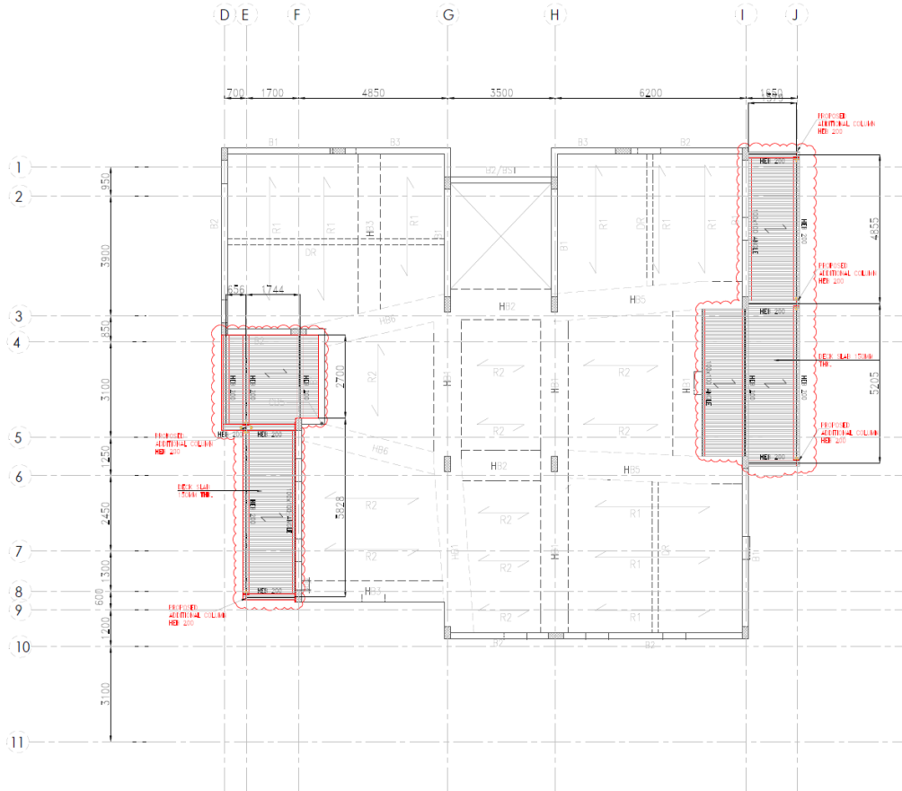
ROOF FLOOR SLAB LAYOUT - AS REVISED
